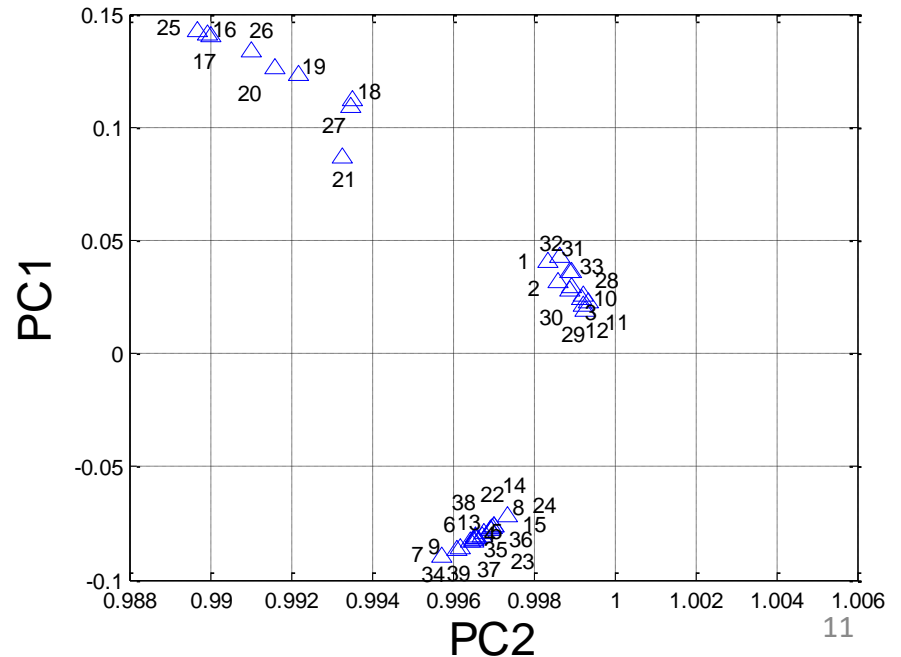
Score plot of the 39 spectrum data (PC1 vs PC2)
