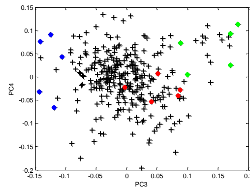
Loadings (chemicals detected)
